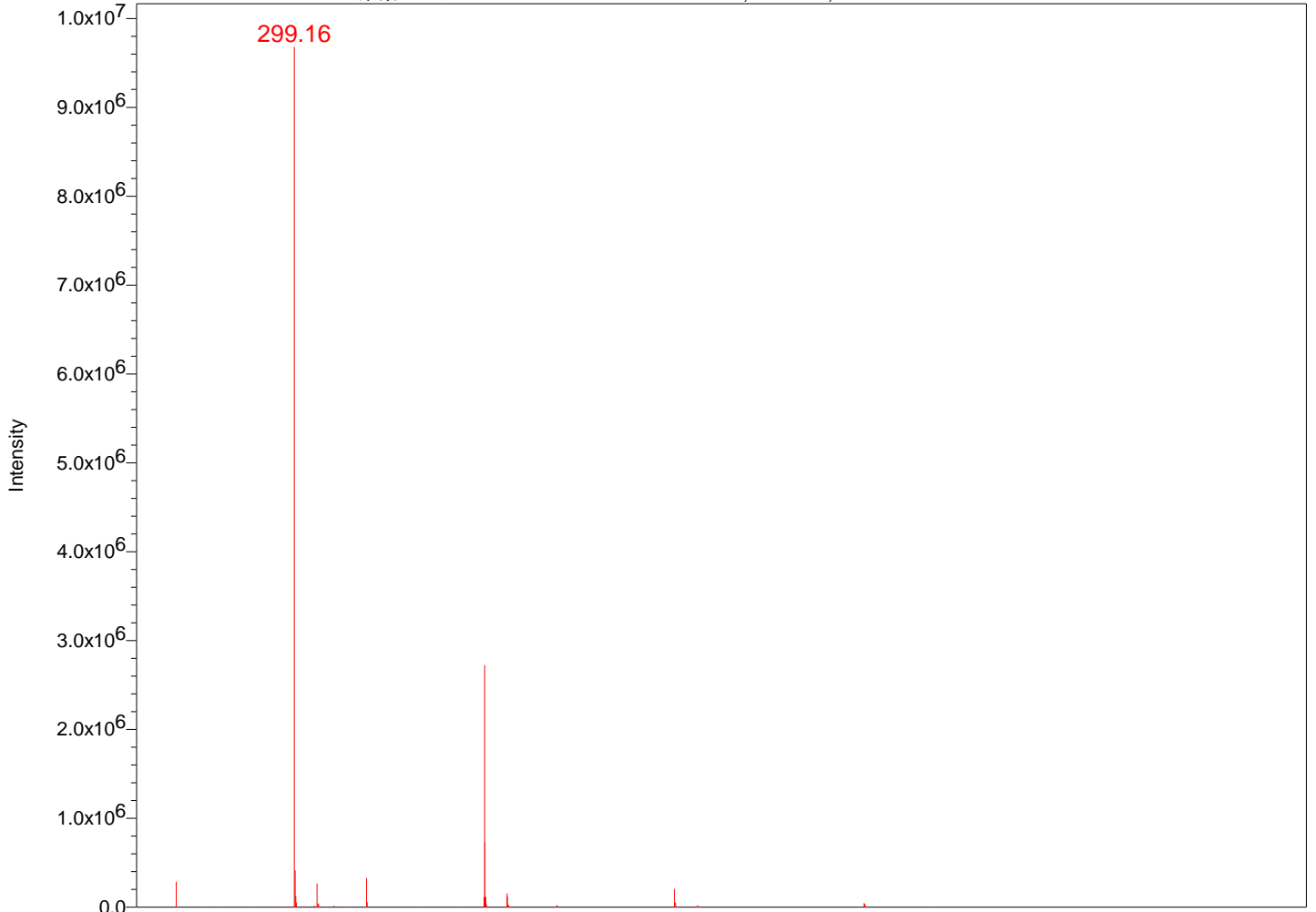
12.259 Extracted -230201山柰素 - SQ 1: MS Scan 1: 50.00-1900.00 ES+, Centroid, CV=30
