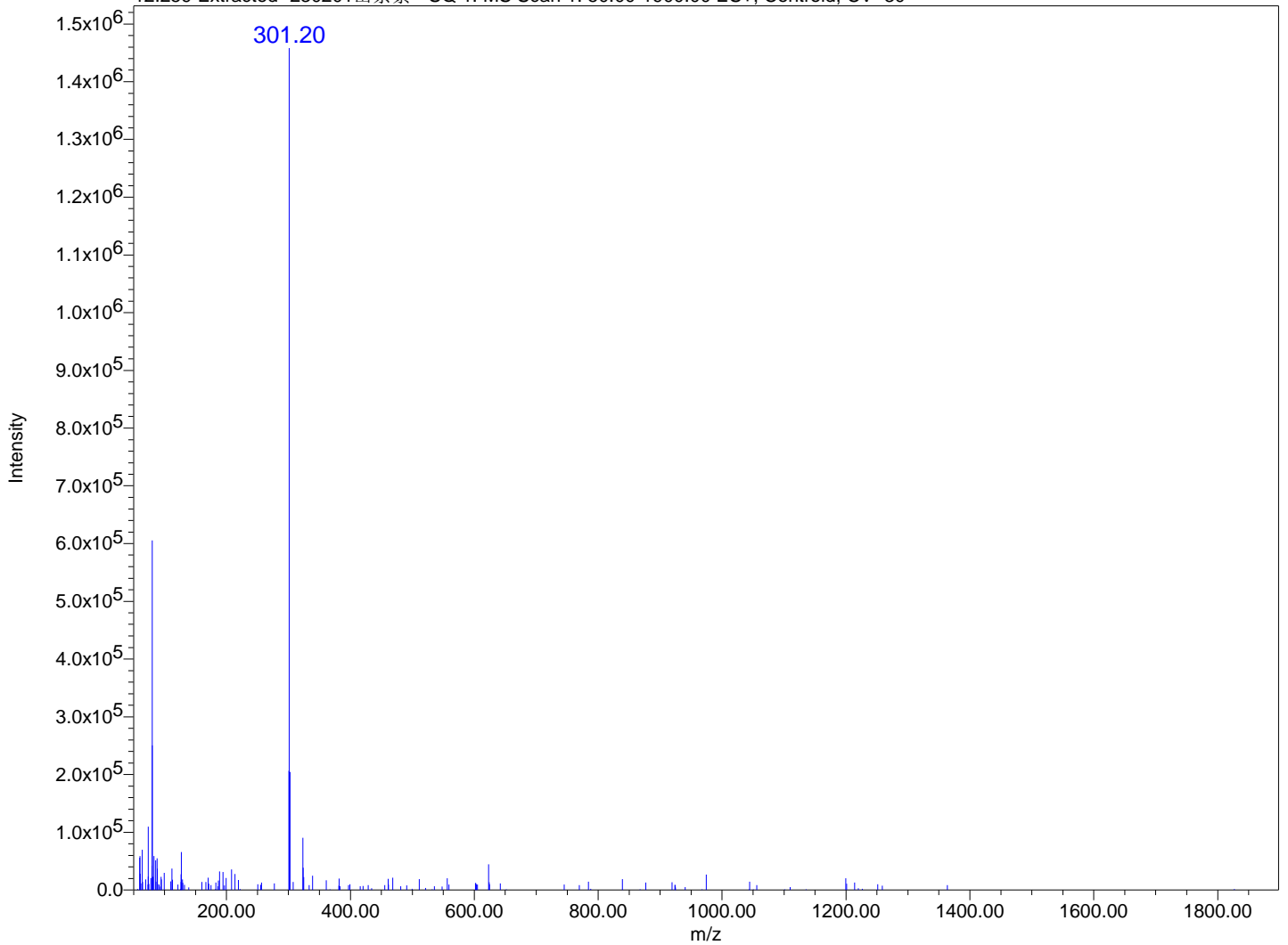
12.259 Extracted -230201山柰素 - SQ 1: MS Scan 1: 50.00-1900.00 ES+, Centroid, CV=30
